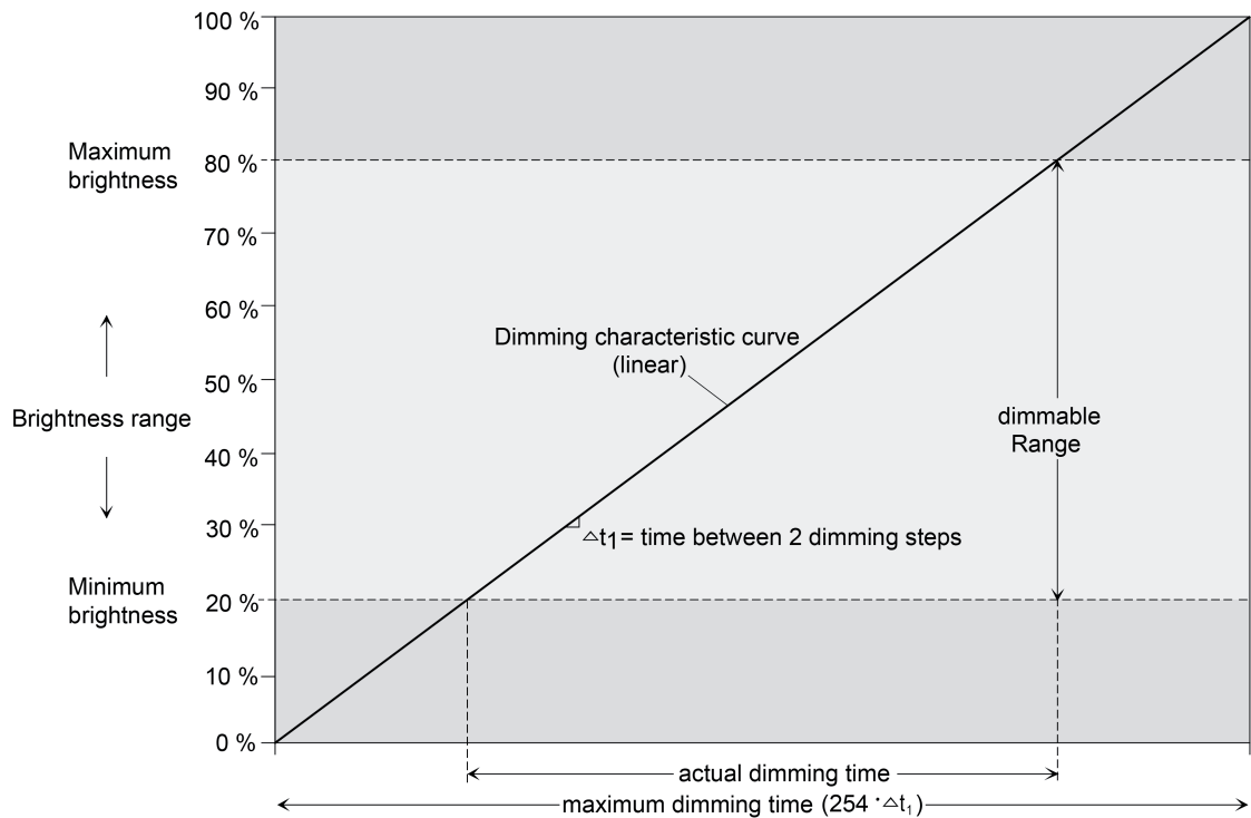
Figure 38: Linear characteristic dimming curve as an example with minimum brightness > 0 % and maximum brightness
