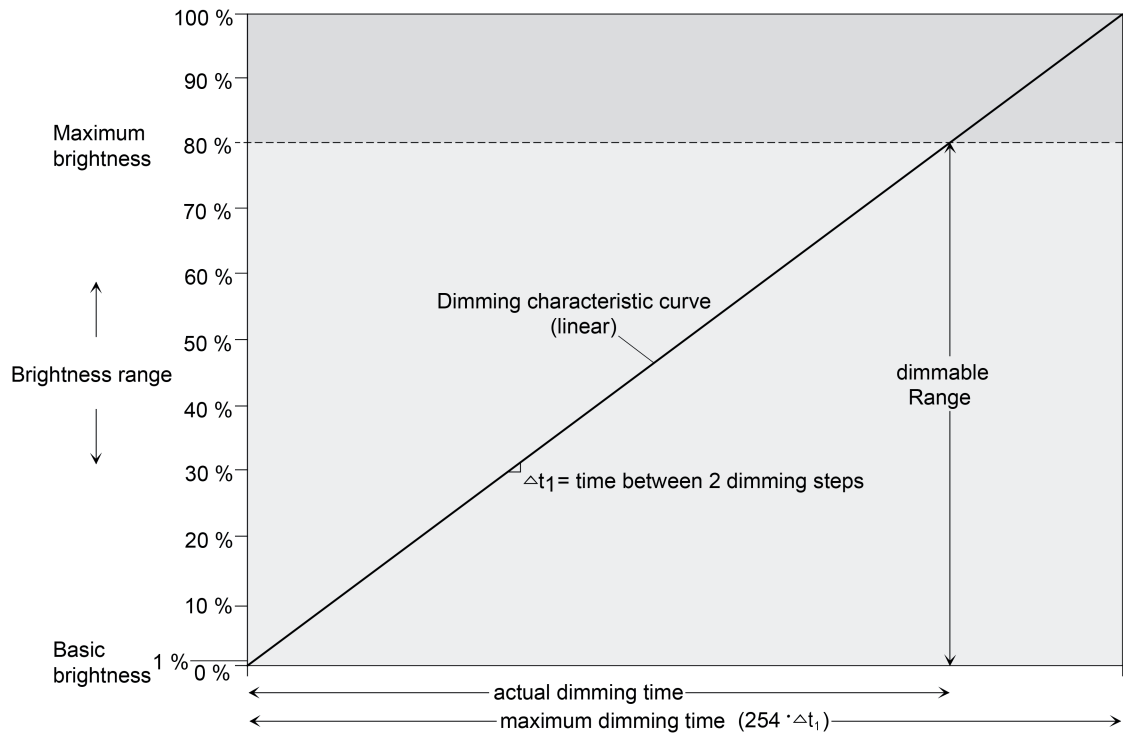
Figure 37: Linear dimming characteristic as an example with basic brightness and maximum brightness
