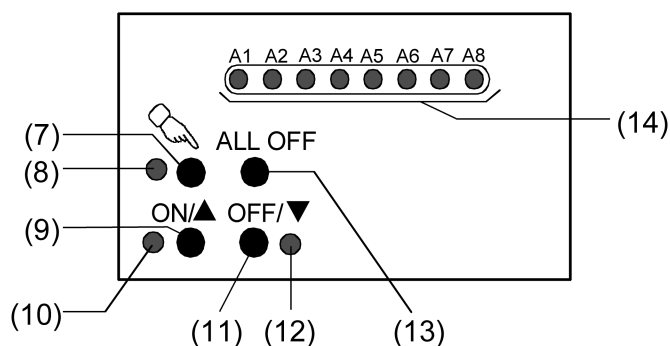
Figure 6: Controls and indicators for manual control
