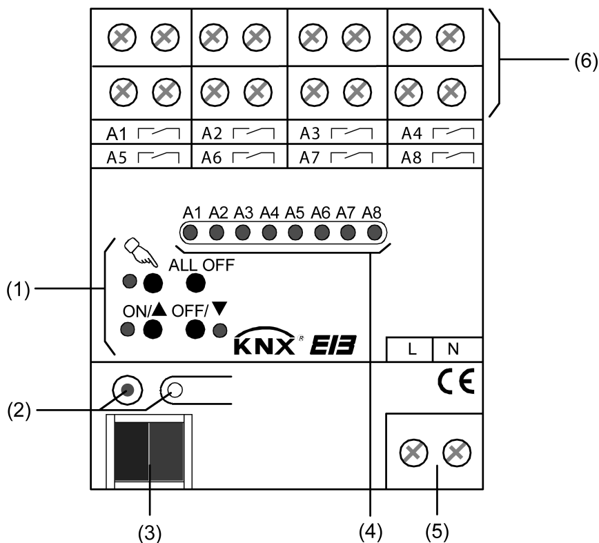
Figure 1: Device components
