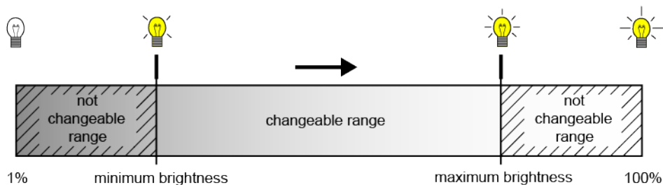
Figure 39: Brightness sequence direction "brighter"
