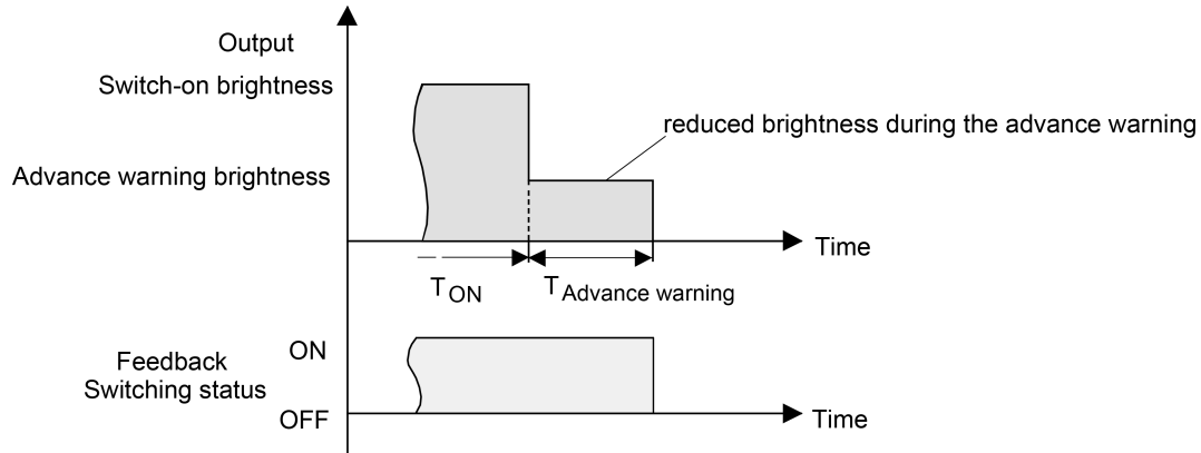
Figure 51: The pre-warning function of the staircase function without soft OFF function
