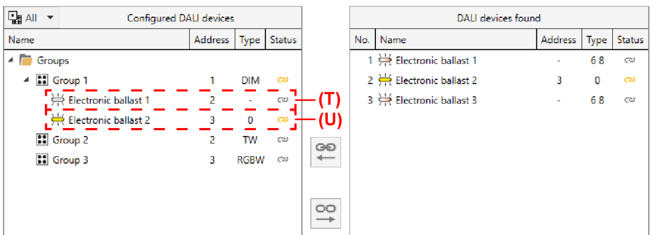
Figure 67: Example of virtual devices of a projected DALI group
