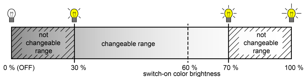
Figure 15: Example of a brightness range with switch-on brightness
