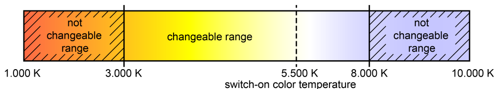
Figure 21: Example of a configured colour temperature range with switch-on colour temperature
