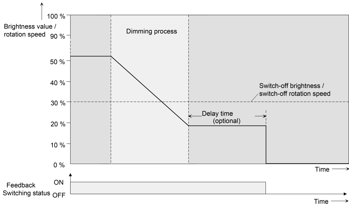
Figure 46: Dimming and switching behaviour of the automatic switch-off function
