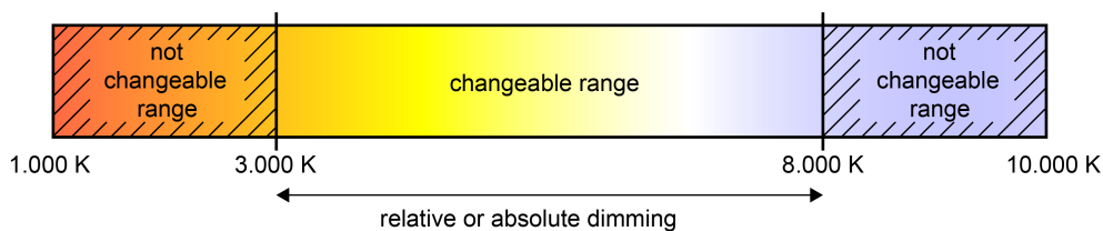
Figure 24: Automatic adjustment of the colour temperature to the set brightness Example with limited brightness and colour temperature range
