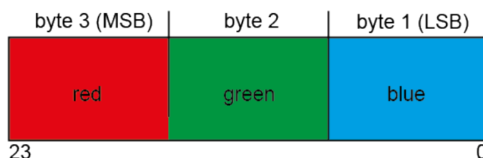
Figure 30: KNX data type "RGB combined" (DPT 232.600)
