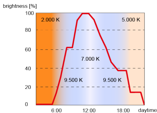
Figure 29: Exemplary daytime colour temperature sequence "Office work"
