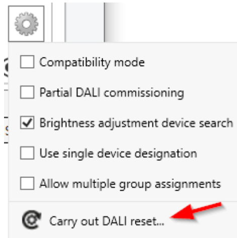
Figure 73: DALI reset command in the context menu of DALI commissioning
