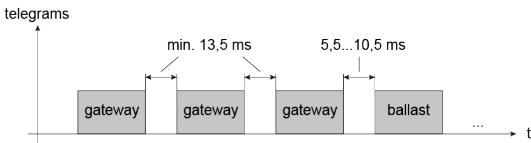
Figure 10: Pause times between DALI commands
