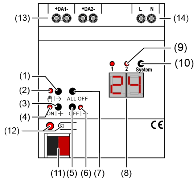
Figure 1: Device components
