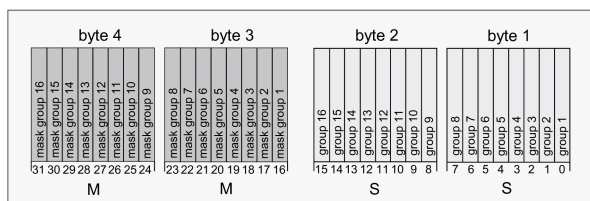
Figure 11: Structure of the objects of the collective feedback, using the example of the object for Groups 1-16
