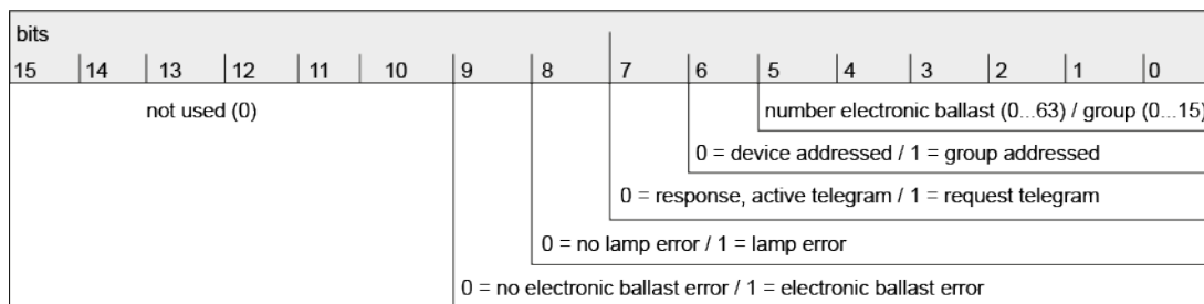
Figure 13: Telegram structure, 2-byte error status
