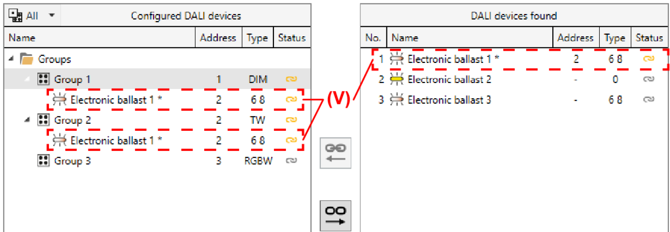
Figure 69: Example for multiple group assignment of a DALI operating device
