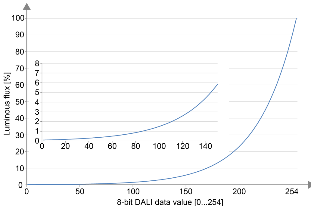
Figure 17: Logarithmic dimming curve in DALI operating devices (relative luminous flux [%] depending on the 8-bit DALI data value [0...254])
