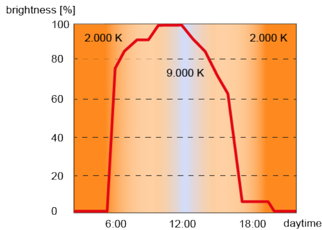
Figure 28: Exemplary daytime colour temperature sequence "Health & Care"
