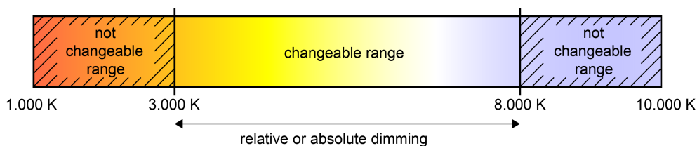
Figure 25: Automatic adjustment of the colour temperature to the set brightness Example with limited colour temperature range
