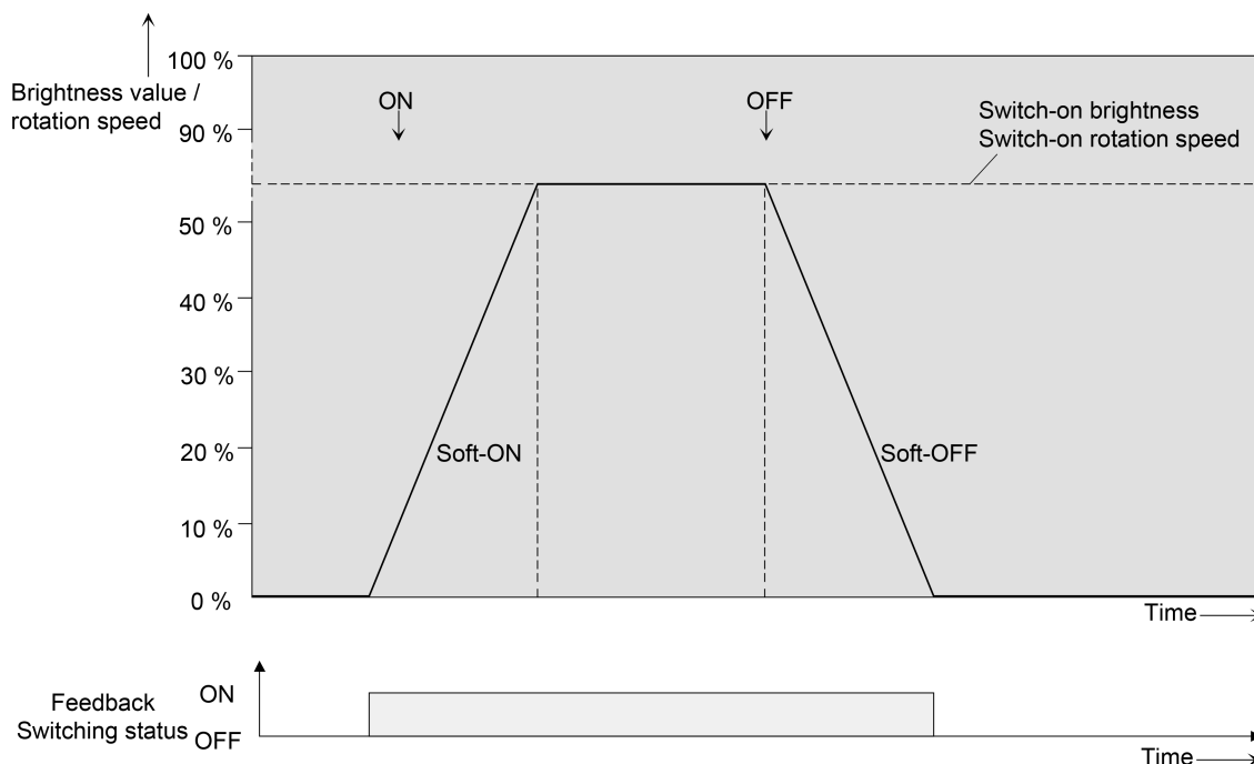
Figure 45: Dimming behaviour of the soft ON/OFF functions as an example with minimum brightness > 0%
