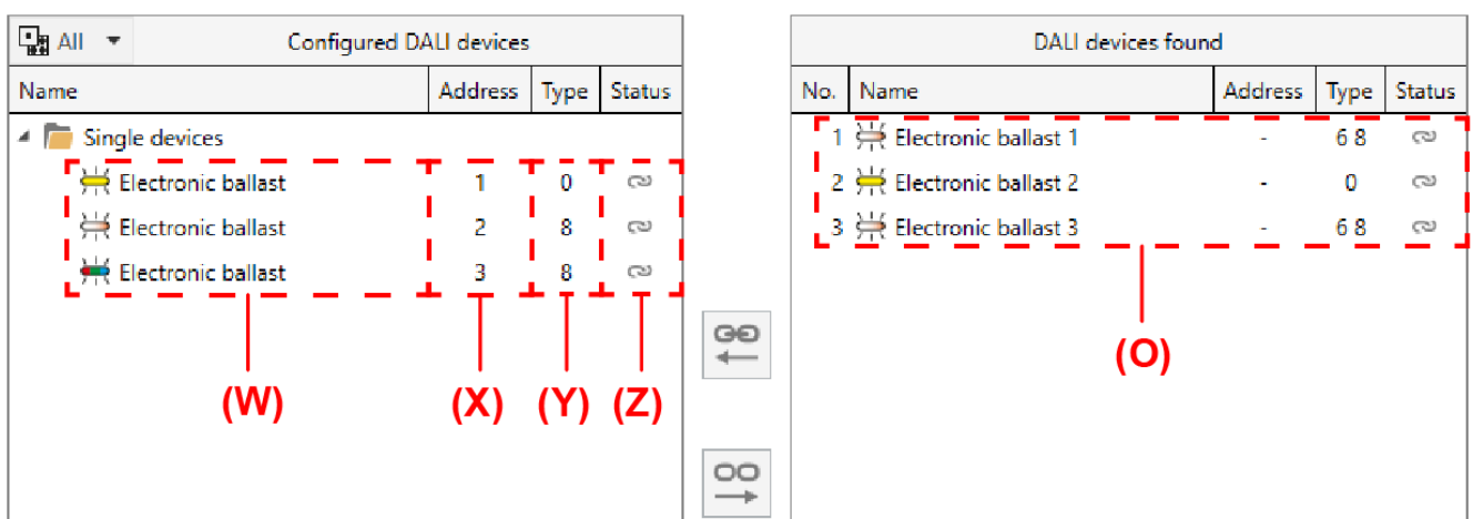
Figure 70: Example of projected DALI single devices in the left display area
