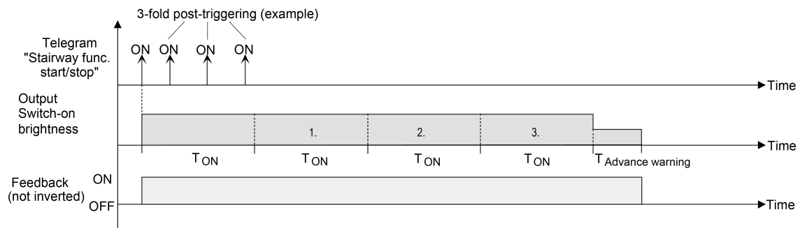
Figure 55: Time extension of the staircase function
