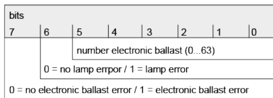
Figure 12: Telegram structure, 1-byte error status
