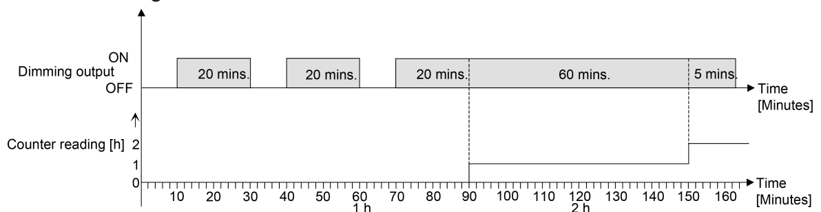
Figure 56: Function of the operating hours counter (using the example of counted hours)
