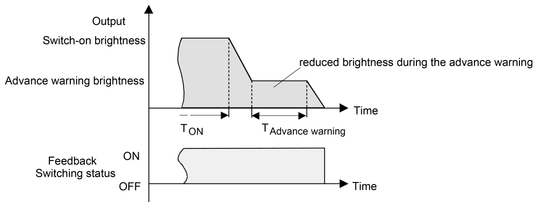
Figure 52: The pre-warning function of the staircase function with soft OFF function (as an example with minimum brightness = 0%)
