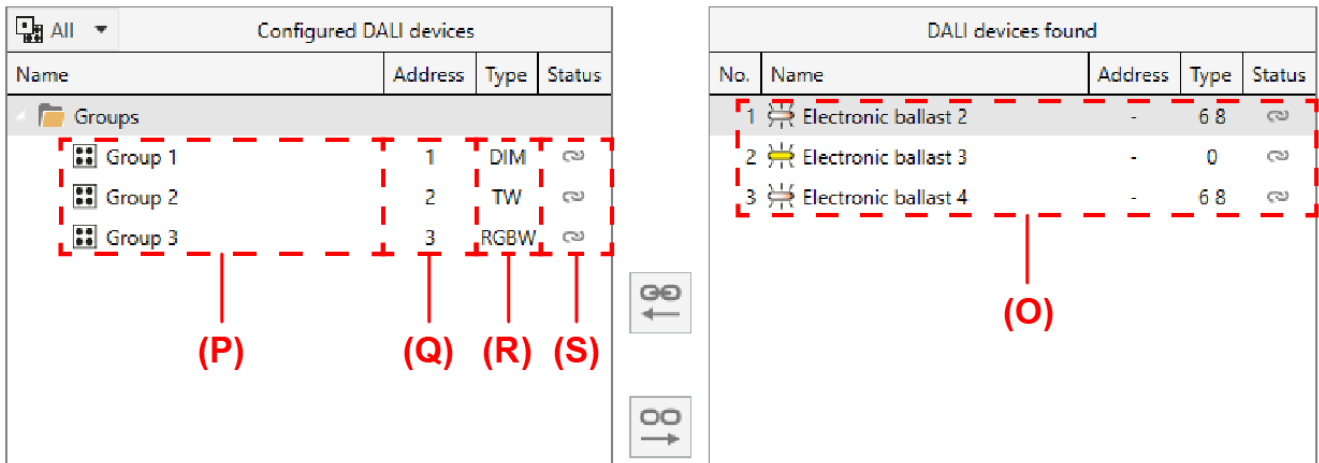
Figure 66: Example of projected DALI groups in the left display area
